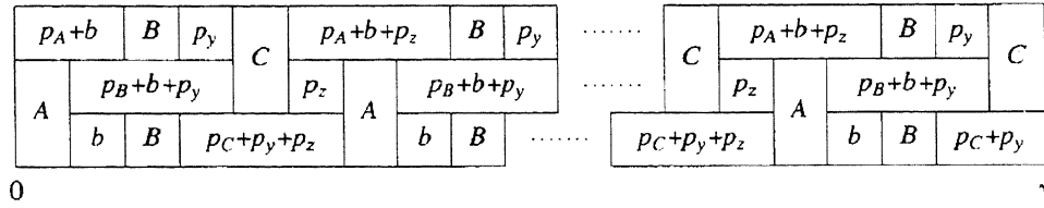
Fig. 4. Structure for P3|fix_j|C_{max} : ABCAB\dots CAB .
